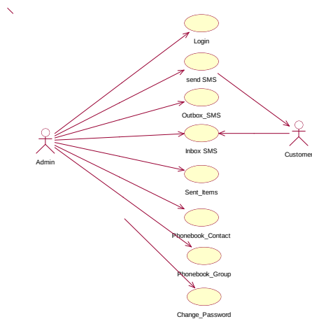
Gambar 2.1 Use Case Diagram SMS Gateway Mega Finance
