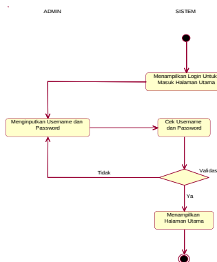
Gambar 2.9 Activity Diagram Login
