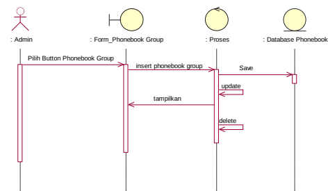
Gambar 2.7 Sequence Diagram Phonebook Group
