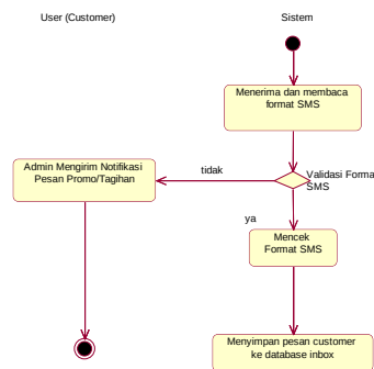
Gambar 2.11 Activity Diagram Customer
