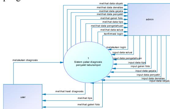
Gambar 3 Context Diagram
