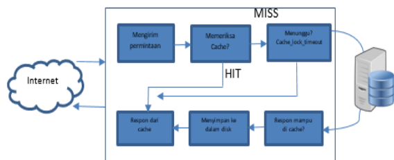
Gambar 2. Proses caching data
