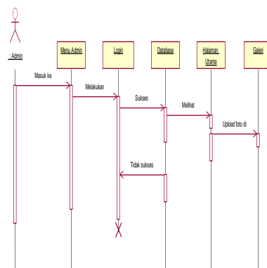
Gambar 10 Sequence Diagram Galeri
