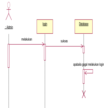
Gambar 7. Sequence Diagram Halaman Admin
