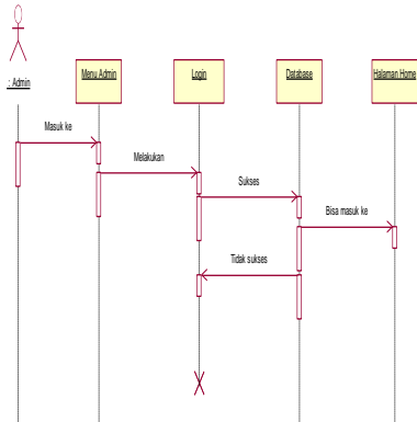
Gambar 9. Sequence Diagram Halaman Home
