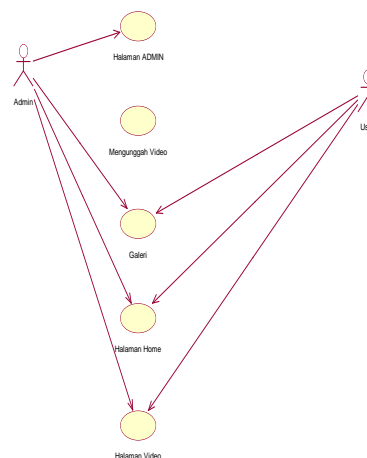
Gambar 1. Use Case Diagram Video
